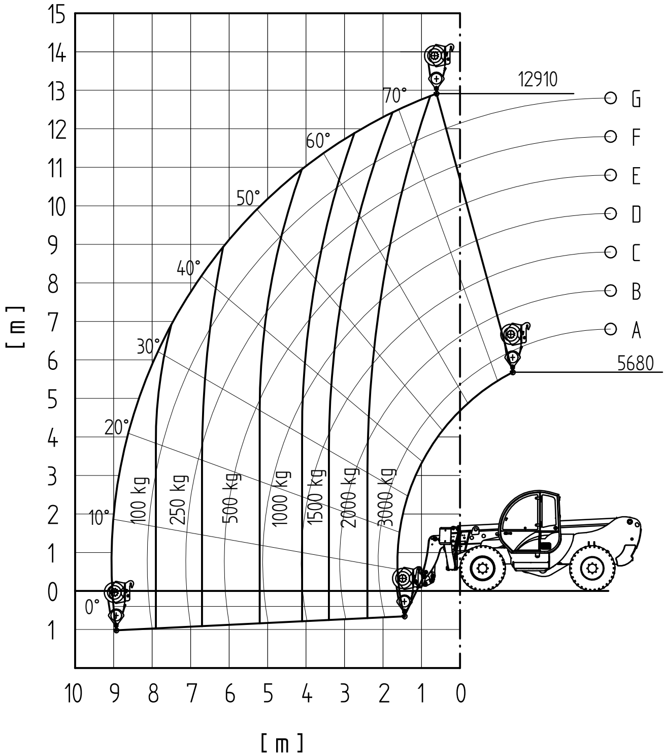
Load Chart with Winch
